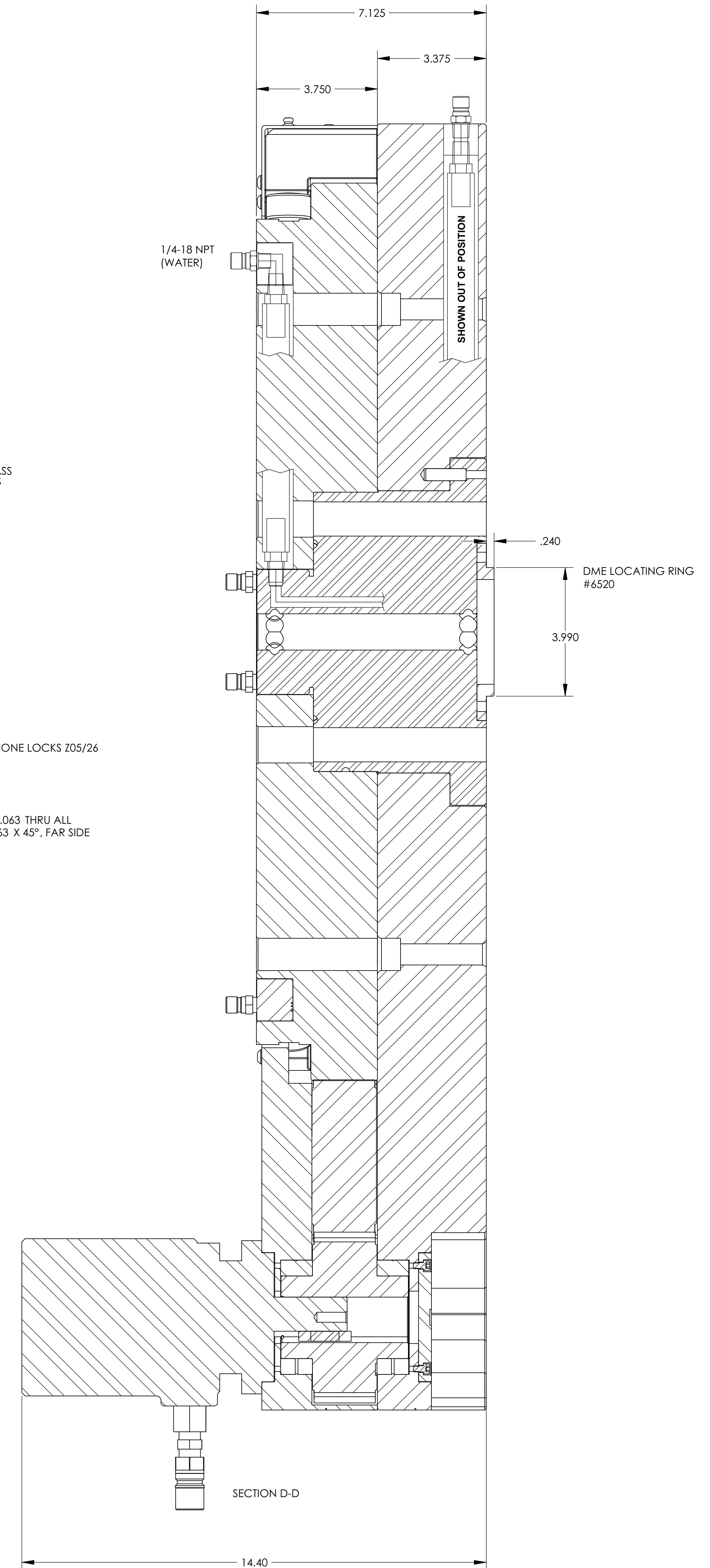
STANDARD MOTOR MOUNTING POSITION
